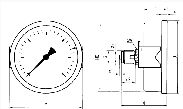
NG 100 – centre back connection, with clamp fixing
