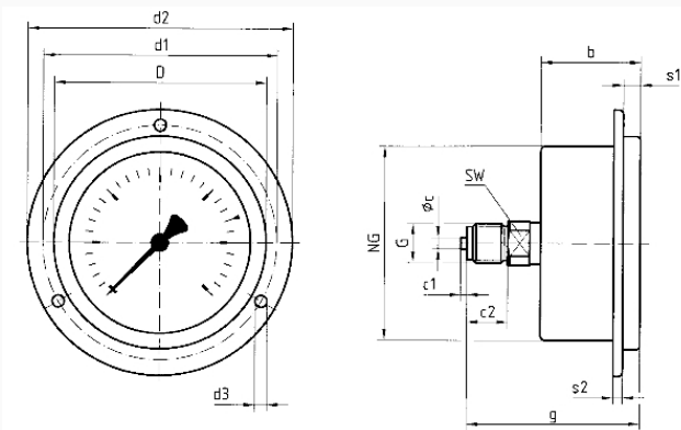
Dimensions (mm)
