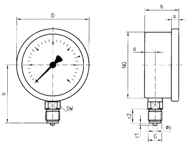
Dimensions (mm)
