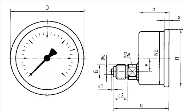
NG 50 – bottom back connection
