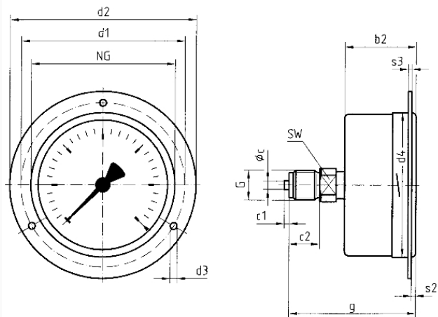
Dimensions (mm)
