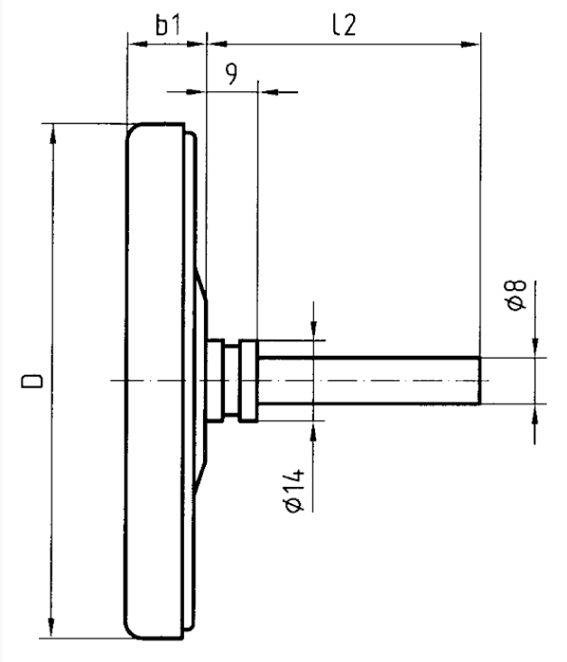
Dimensions (mm)
