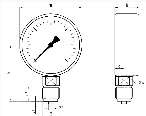
NG 80/100 – Anschluss radial
